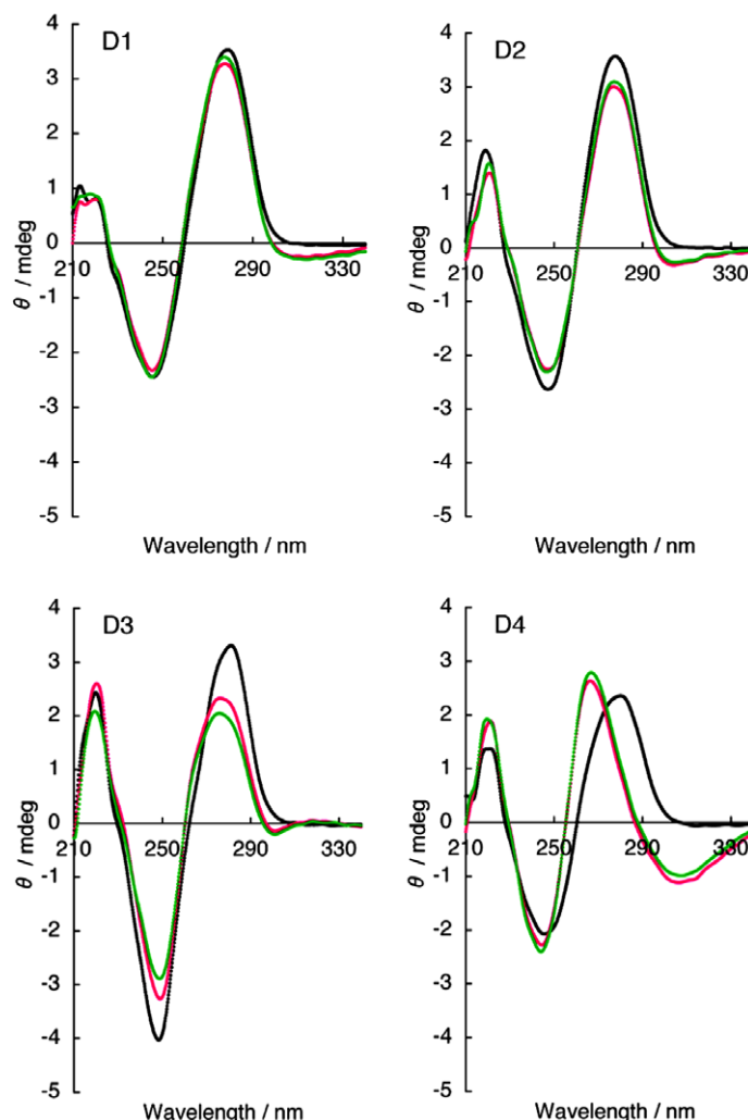
Figure 3. CD spectra of unmodified (black), Mal-modified (red), and Lac-modified (green) DNA ( D1–4 ). The measurements were performed under the following conditions: 0.8 \mu M duplex, 10 mM \text{Na}_2\text{HPO}_4/\text{NaH}_2\text{PO}_4 , 10 mM NaCl, and 1 mM EDTA, pH 7.0, 25 ^\circ\text{C} .
