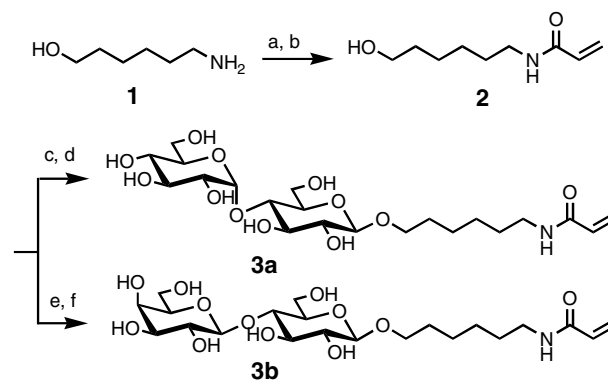
Scheme 1. Reagents and conditions: (a) acryloyl chloride, triethylamine, CH 2 Cl 2 , 45 °C to rt; (b) 2 M NaOH, EtOH, rt, 69% (two steps); (c) maltose octaacetate, BF 3 ·(C 2 H 5 ) 2 O, dry CH 2 Cl 2 , rt; (d) NaOMe, MeOH, rt, 63% (two steps); (e) heptaacetyl-α-bromolactose, AgClO 4 , Ag 2 CO 3 , dry CH 2 Cl 2 , 0 °C; (f) NaOMe, MeOH, rt, 32% (two steps).
